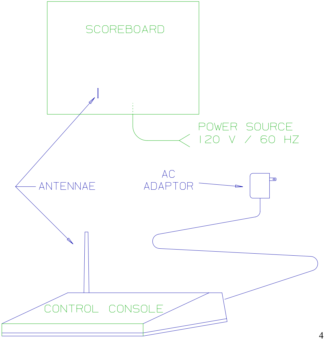
figure 4 SYSTEM LAYOUT
