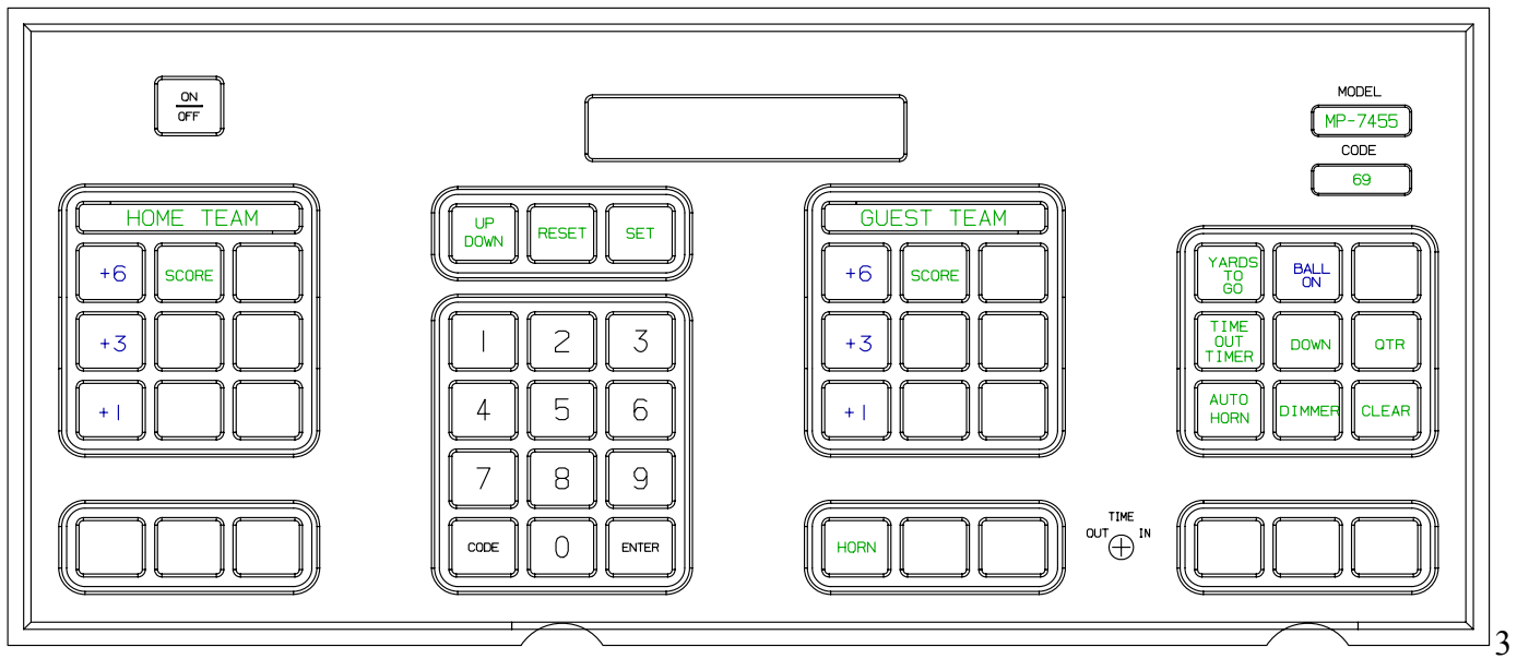
figure 3 CONSOLE KEYBOARD
